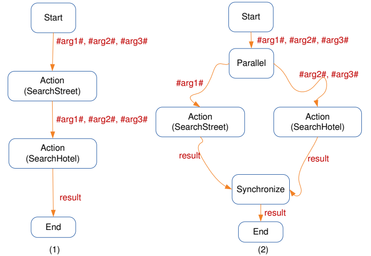
Fig. 8: Workflow examples.
