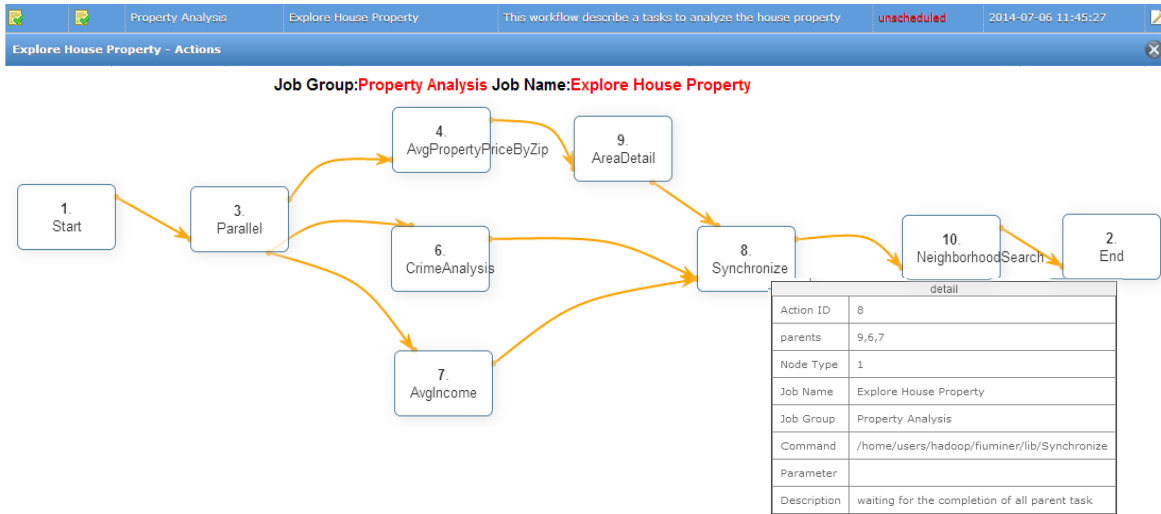
Fig. 9: The workflow of searching for house properties with a good appreciation potential. All the sub-tasks in the workflow are scheduled by FIU-Miner and are executed in the distributed environment.
