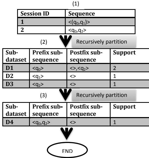
Fig. 5: An example illustrating the PrefixSpan algorithm.
