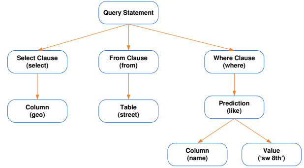
Fig. 4: The syntax tree for a MapQL statement “SELECT geo FROM street WHERE name LIKE ‘sw 8th’;”.
