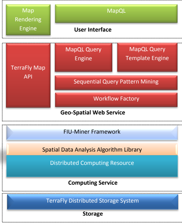
Fig. 3: The system overview.
